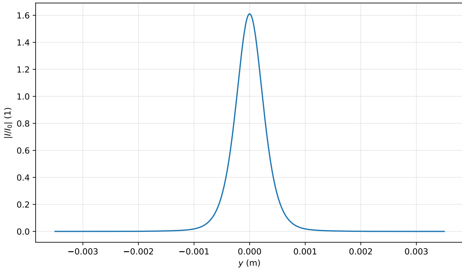
Intensity profile I(x = 0, y, z = 2.627)/I_0 , P_{in}=0.9P_{cr} , artificial time
